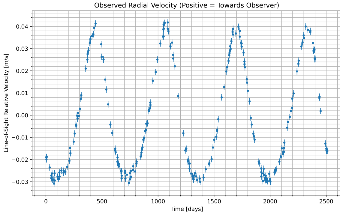
Figure 1: We have isolated the radial velocity of the host star due to the candidate planet. Data begins at UTC 2090-05-18/05:24. Positive values indicate the velocity at which the star is moving towards us; negative indicate the velocity at which it is moving away.
