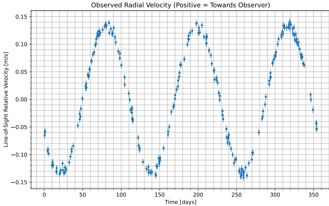
Figure 1: We have isolated the radial velocity of the host star due to the candidate planet. Data begins at UTC 2075-07-17/23:39. Positive values indicate the velocity at which the star is moving towards us; negative indicate the velocity at which it is moving away.
