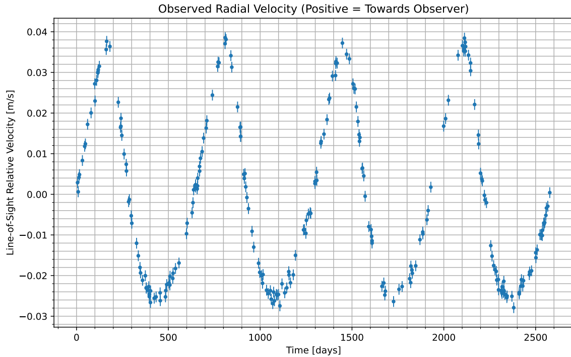
Figure 1: We have isolated the radial velocity of the host star due to the candidate planet. Data begins at UTC 2072-09-29/22:44. Positive values indicate the velocity at which the star is moving towards us; negative indicate the velocity at which it is moving away.
