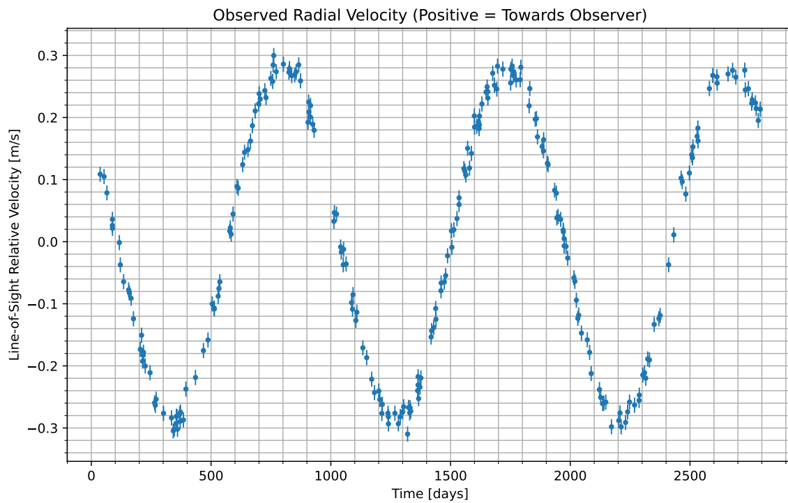
Figure 1: We have isolated the radial velocity of the host star due to the candidate planet. Data begins at UTC 2086-03-07/15:56. Positive values indicate the velocity at which the star is moving towards us; negative indicate the velocity at which it is moving away.
