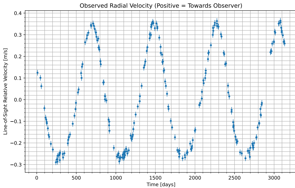
Figure 1: We have isolated the radial velocity of the host star due to the candidate planet. Data begins at UTC 2065-03-15/07:52. Positive values indicate the velocity at which the star is moving towards us; negative indicate the velocity at which it is moving away.
