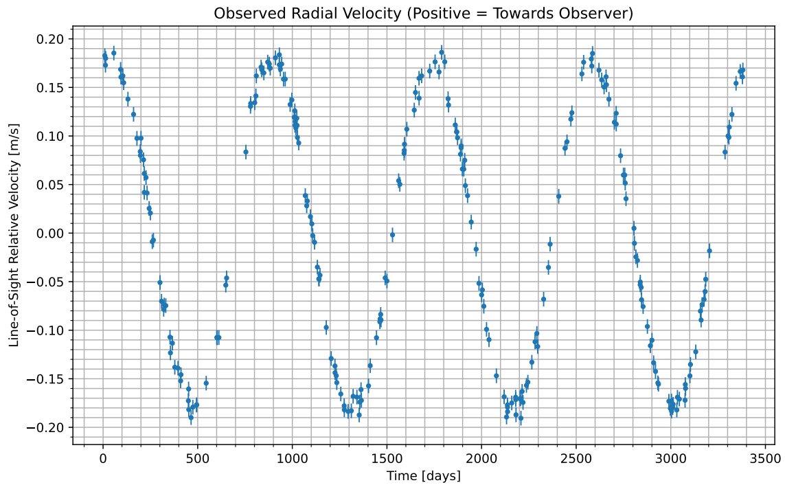
Figure 1: We have isolated the radial velocity of the host star due to the candidate planet. Data begins at UTC 2075-09-04/13:49. Positive values indicate the velocity at which the star is moving towards us; negative indicate the velocity at which it is moving away.
