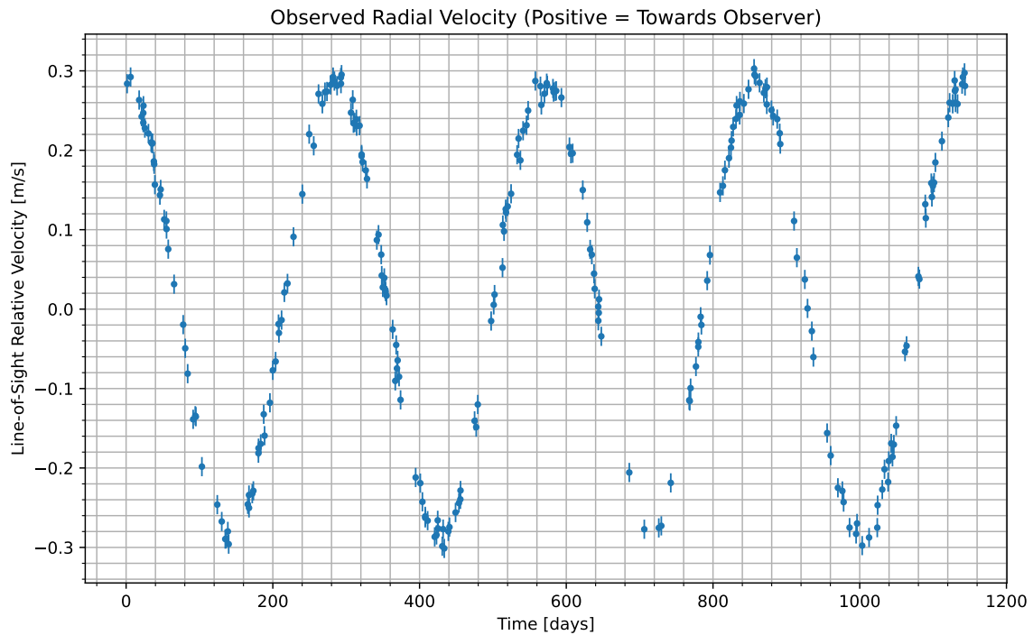
Figure 1: We have isolated the radial velocity of the host star due to the candidate planet. Data begins at UTC 2079-07-16/18:48. Positive values indicate the velocity at which the star is moving towards us; negative indicate the velocity at which it is moving away.
