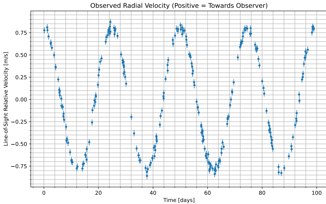
Figure 1: We have isolated the radial velocity of the host star due to the candidate planet. Data begins at UTC 2070-10-11/22:29. Positive values indicate the velocity at which the star is moving towards us; negative indicate the velocity at which it is moving away.
