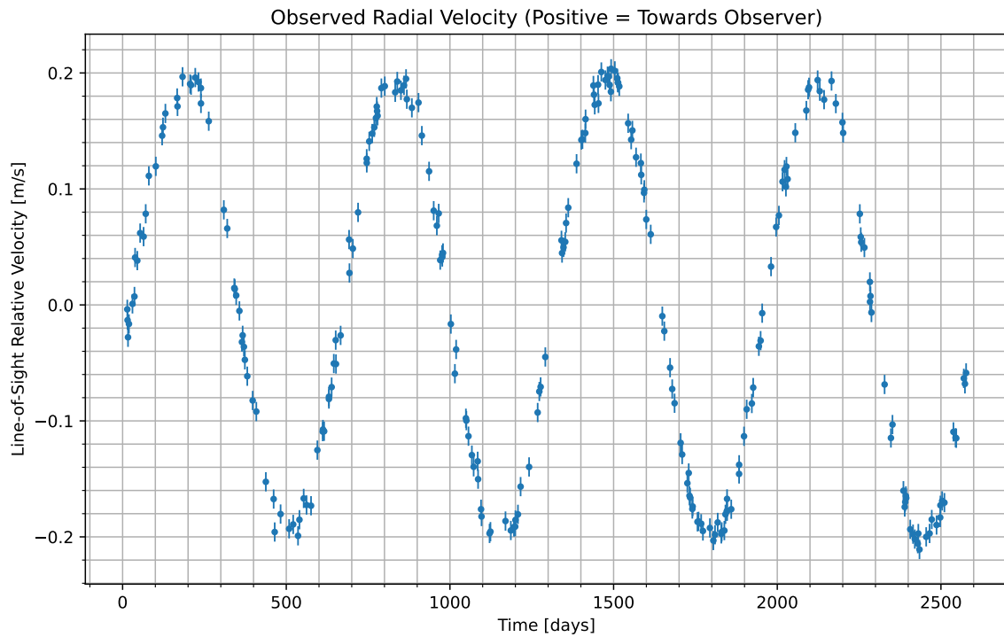
Figure 1: We have isolated the radial velocity of the host star due to the candidate planet. Data begins at UTC 2067-02-05/12:39. Positive values indicate the velocity at which the star is moving towards us; negative indicate the velocity at which it is moving away.
