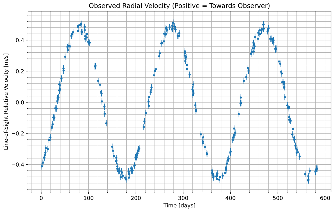
Figure 1: We have isolated the radial velocity of the host star due to the candidate planet. Data begins at UTC 2087-10-16/06:04. Positive values indicate the velocity at which the star is moving towards us; negative indicate the velocity at which it is moving away.
