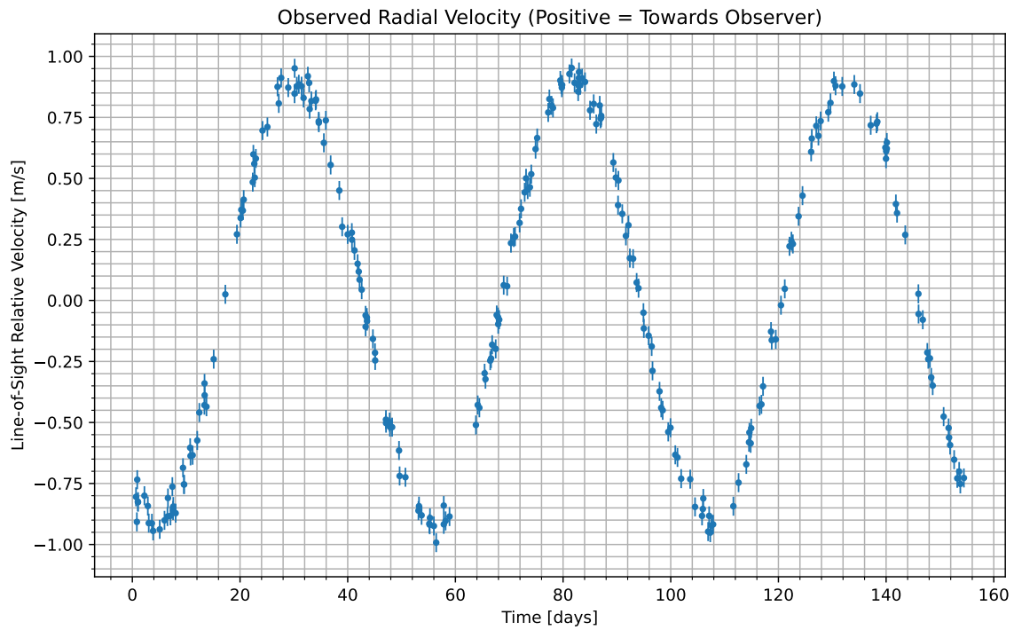
Figure 1: We have isolated the radial velocity of the host star due to the candidate planet. Data begins at UTC 2077-04-13/04:33. Positive values indicate the velocity at which the star is moving towards us; negative indicate the velocity at which it is moving away.
