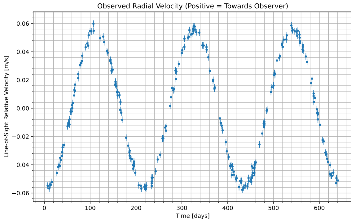
Figure 1: We have isolated the radial velocity of the host star due to the candidate planet. Data begins at UTC 2075-07-22/01:23. Positive values indicate the velocity at which the star is moving towards us; negative indicate the velocity at which it is moving away.
