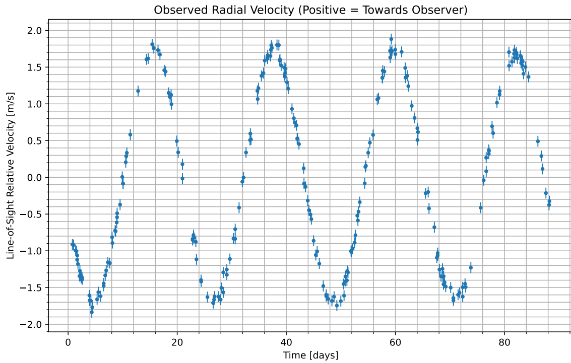
Figure 1: We have isolated the radial velocity of the host star due to the candidate planet. Data begins at UTC 2071-09-17/03:51. Positive values indicate the velocity at which the star is moving towards us; negative indicate the velocity at which it is moving away.
