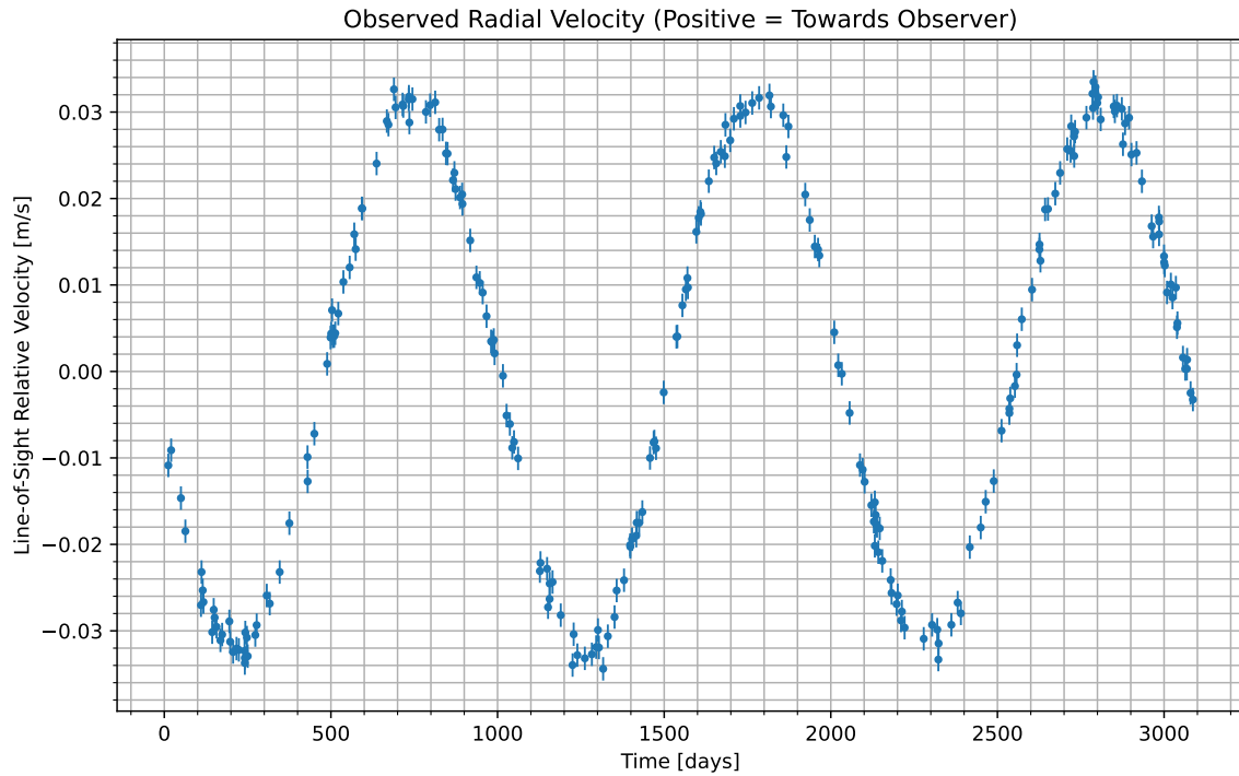
Figure 1: We have isolated the radial velocity of the host star due to the candidate planet. Data begins at UTC 2065-08-13/17:13. Positive values indicate the velocity at which the star is moving towards us; negative indicate the velocity at which it is moving away.
