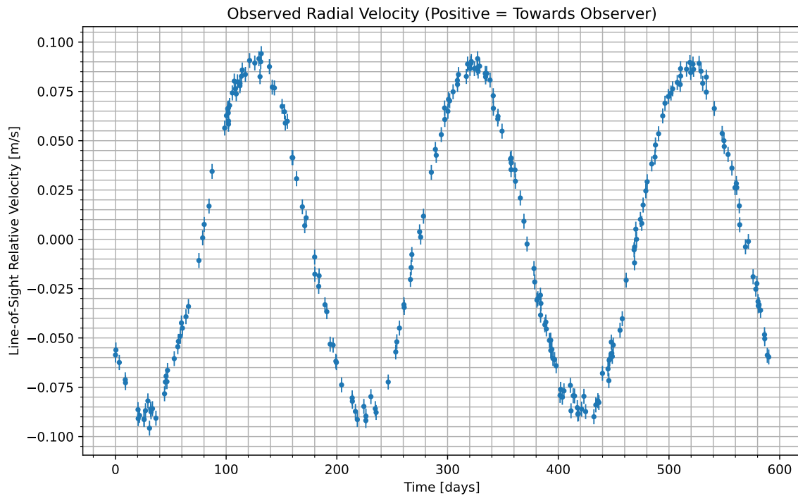
Figure 1: We have isolated the radial velocity of the host star due to the candidate planet. Data begins at UTC 2090-05-29/21:55. Positive values indicate the velocity at which the star is moving towards us; negative indicate the velocity at which it is moving away.
