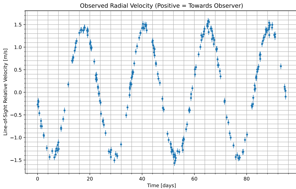
Figure 1: We have isolated the radial velocity of the host star due to the candidate planet. Data begins at UTC 2085-09-21/13:06. Positive values indicate the velocity at which the star is moving towards us; negative indicate the velocity at which it is moving away.
