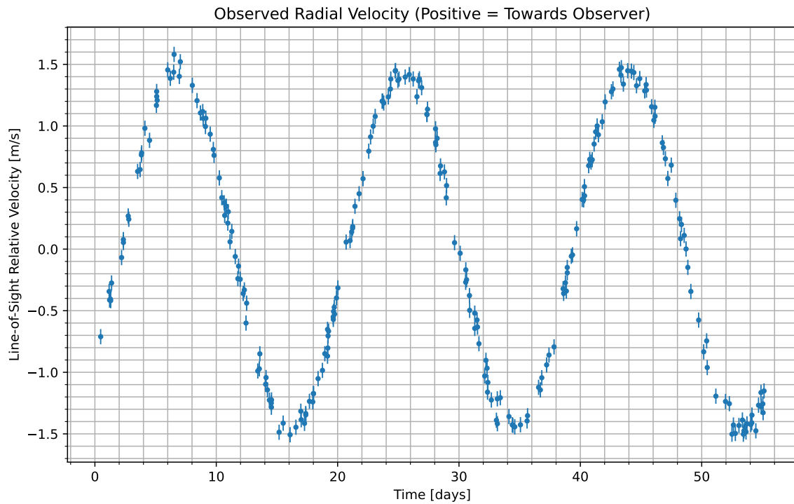
Figure 1: We have isolated the radial velocity of the host star due to the candidate planet. Data begins at UTC 2078-04-14/13:34. Positive values indicate the velocity at which the star is moving towards us; negative indicate the velocity at which it is moving away.
