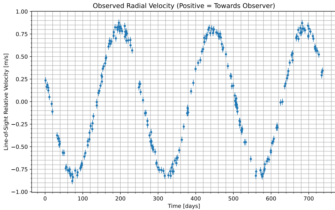
Figure 1: We have isolated the radial velocity of the host star due to the candidate planet. Data begins at UTC 2096-05-02/09:10. Positive values indicate the velocity at which the star is moving towards us; negative indicate the velocity at which it is moving away.
