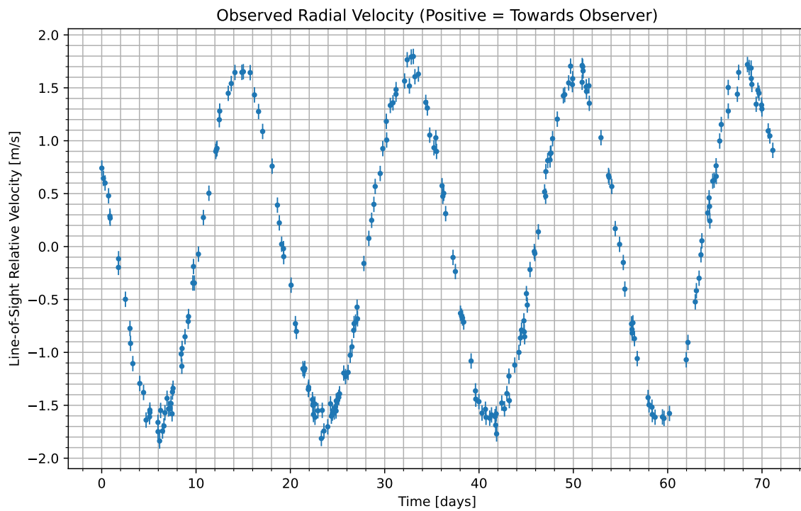
Figure 1: We have isolated the radial velocity of the host star due to the candidate planet. Data begins at UTC 2075-12-21/15:12. Positive values indicate the velocity at which the star is moving towards us; negative indicate the velocity at which it is moving away.
