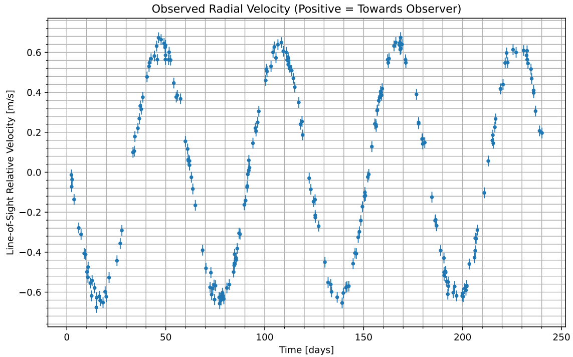
Figure 1: We have isolated the radial velocity of the host star due to the candidate planet. Data begins at UTC 2088-04-19/14:20. Positive values indicate the velocity at which the star is moving towards us; negative indicate the velocity at which it is moving away.
