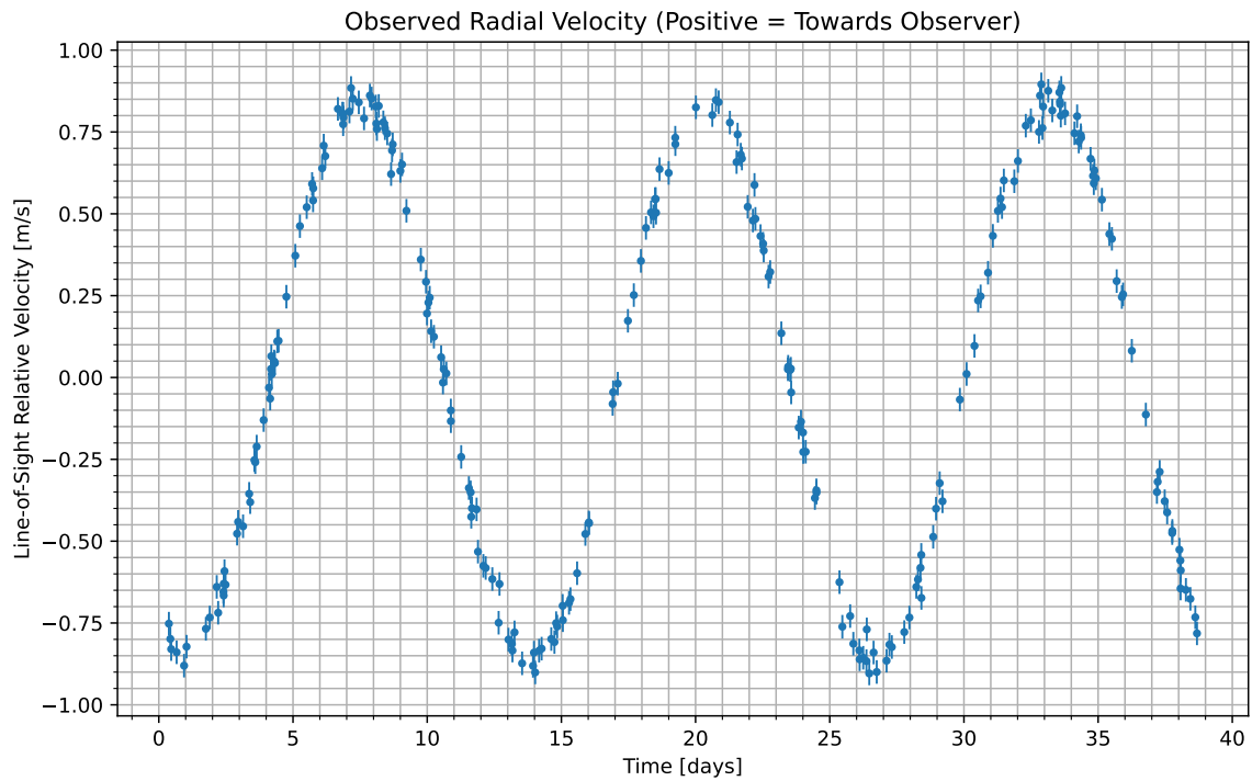
Figure 1: We have isolated the radial velocity of the host star due to the candidate planet. Data begins at UTC 2099-08-14/15:33. Positive values indicate the velocity at which the star is moving towards us; negative indicate the velocity at which it is moving away.
