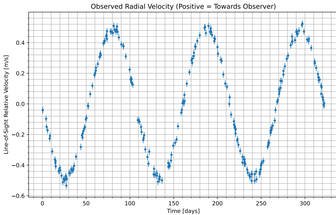
Figure 1: We have isolated the radial velocity of the host star due to the candidate planet. Data begins at UTC 2092-03-14/19:02. Positive values indicate the velocity at which the star is moving towards us; negative indicate the velocity at which it is moving away.
