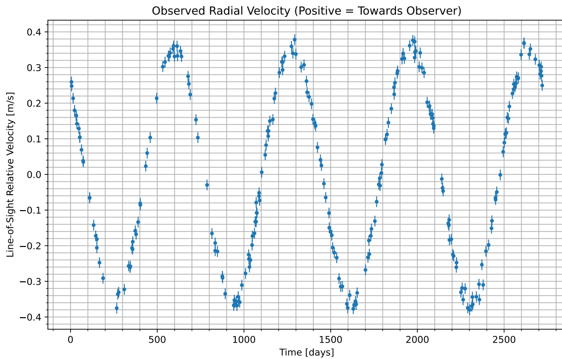
Figure 1: We have isolated the radial velocity of the host star due to the candidate planet. Data begins at UTC 2082-02-05/21:57. Positive values indicate the velocity at which the star is moving towards us; negative indicate the velocity at which it is moving away.
