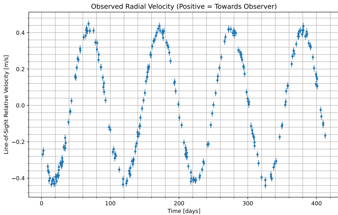
Figure 1: We have isolated the radial velocity of the host star due to the candidate planet. Data begins at UTC 2092-02-29/22:41. Positive values indicate the velocity at which the star is moving towards us; negative indicate the velocity at which it is moving away.
