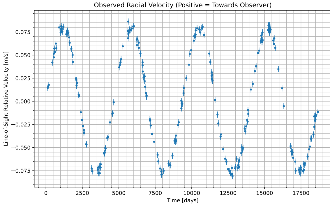
Figure 1: We have isolated the radial velocity of the host star due to the candidate planet. Data begins at UTC 2034-10-31/17:27. Positive values indicate the velocity at which the star is moving towards us; negative indicate the velocity at which it is moving away.
