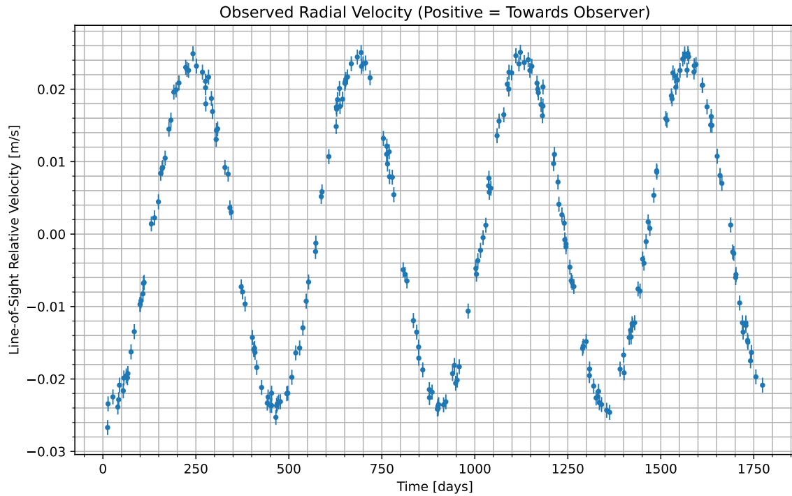
Figure 1: We have isolated the radial velocity of the host star due to the candidate planet. Data begins at UTC 2083-08-15/06:42. Positive values indicate the velocity at which the star is moving towards us; negative indicate the velocity at which it is moving away.
