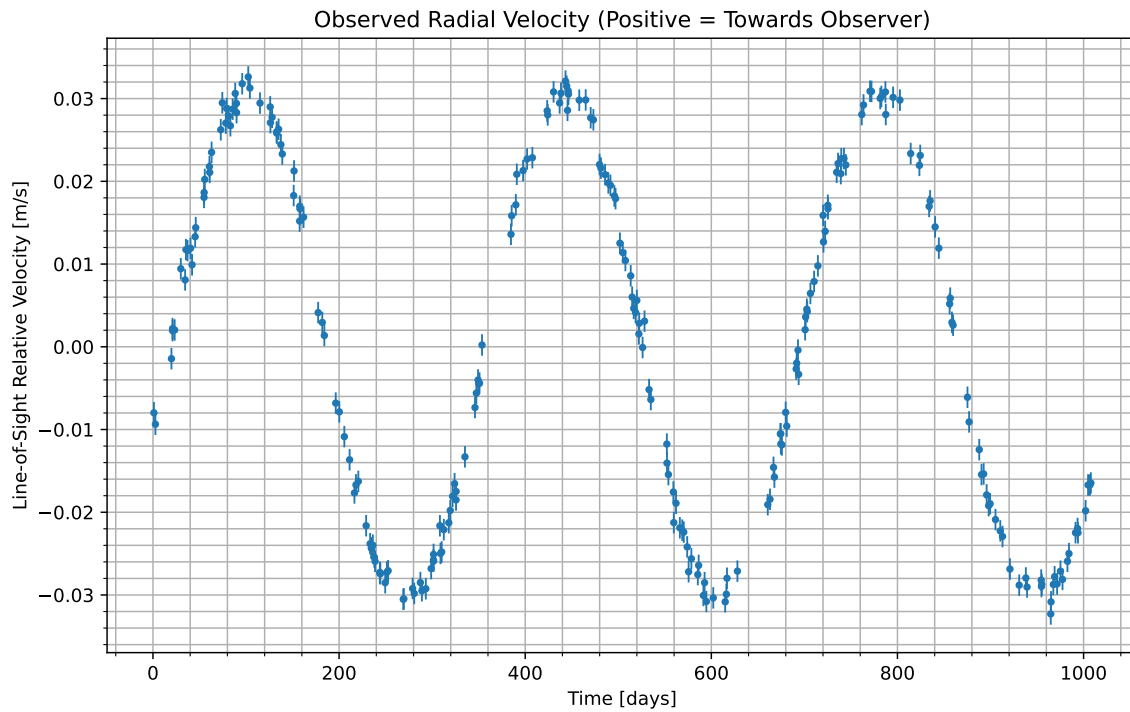
Figure 1: We have isolated the radial velocity of the host star due to the candidate planet. Data begins at UTC 2088-11-03/18:31. Positive values indicate the velocity at which the star is moving towards us; negative indicate the velocity at which it is moving away.
