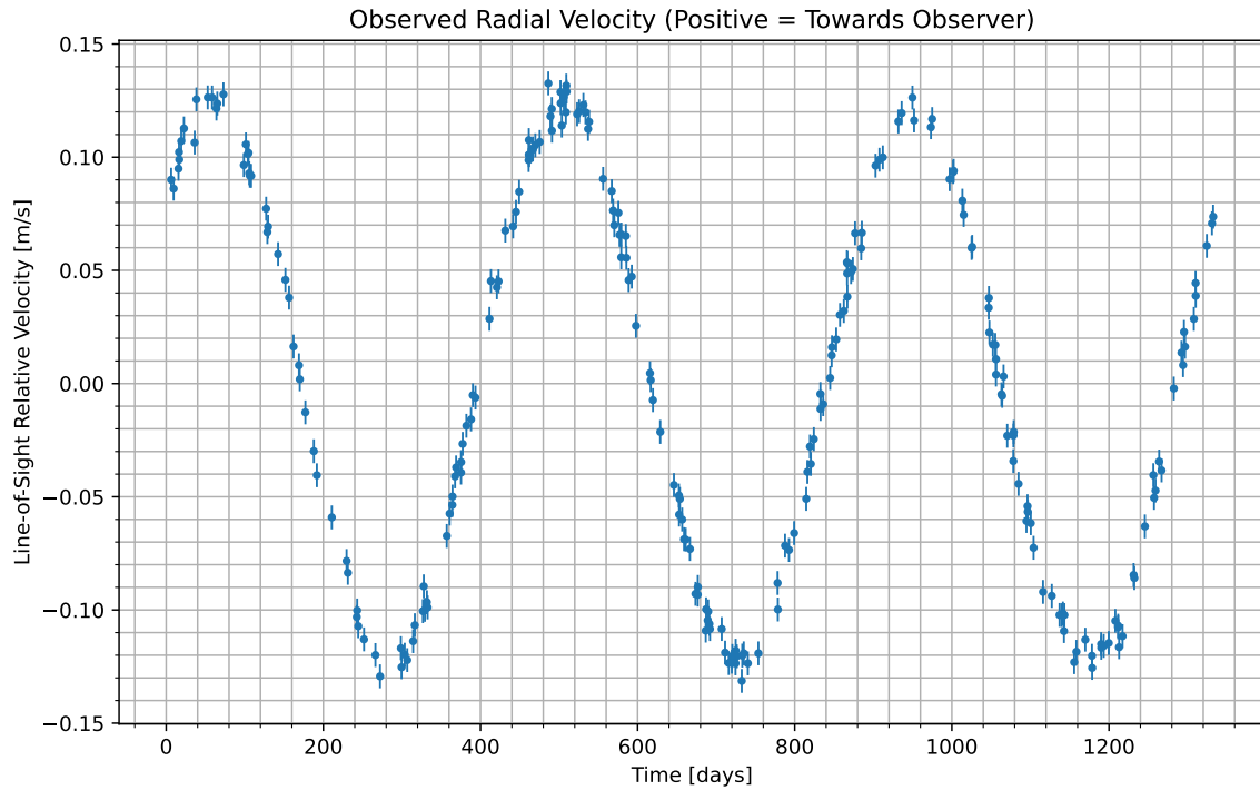
Figure 1: We have isolated the radial velocity of the host star due to the candidate planet. Data begins at UTC 2086-03-31/00:27. Positive values indicate the velocity at which the star is moving towards us; negative indicate the velocity at which it is moving away.
