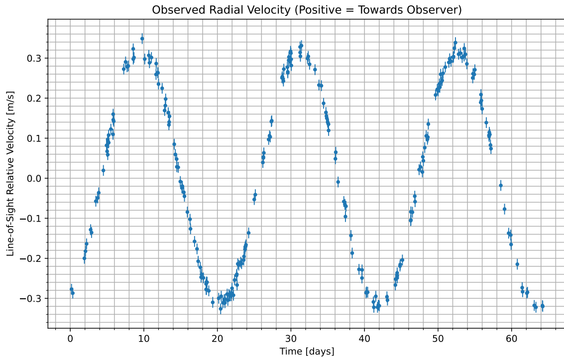
Figure 1: We have isolated the radial velocity of the host star due to the candidate planet. Data begins at UTC 2077-11-18/09:55. Positive values indicate the velocity at which the star is moving towards us; negative indicate the velocity at which it is moving away.
