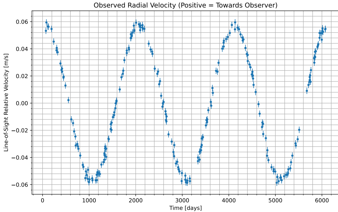
Figure 1: We have isolated the radial velocity of the host star due to the candidate planet. Data begins at UTC 2061-01-04/05:32. Positive values indicate the velocity at which the star is moving towards us; negative indicate the velocity at which it is moving away.
