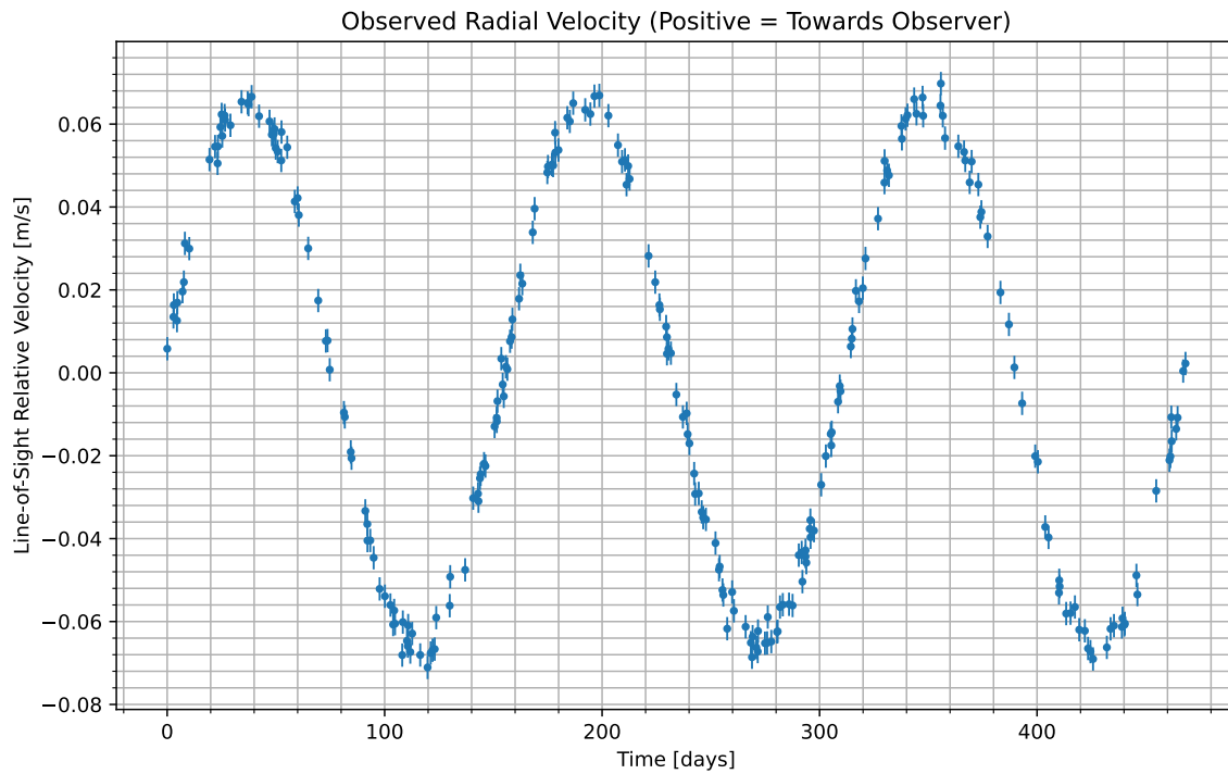
Figure 1: We have isolated the radial velocity of the host star due to the candidate planet. Data begins at UTC 2069-05-06/08:34. Positive values indicate the velocity at which the star is moving towards us; negative indicate the velocity at which it is moving away.
