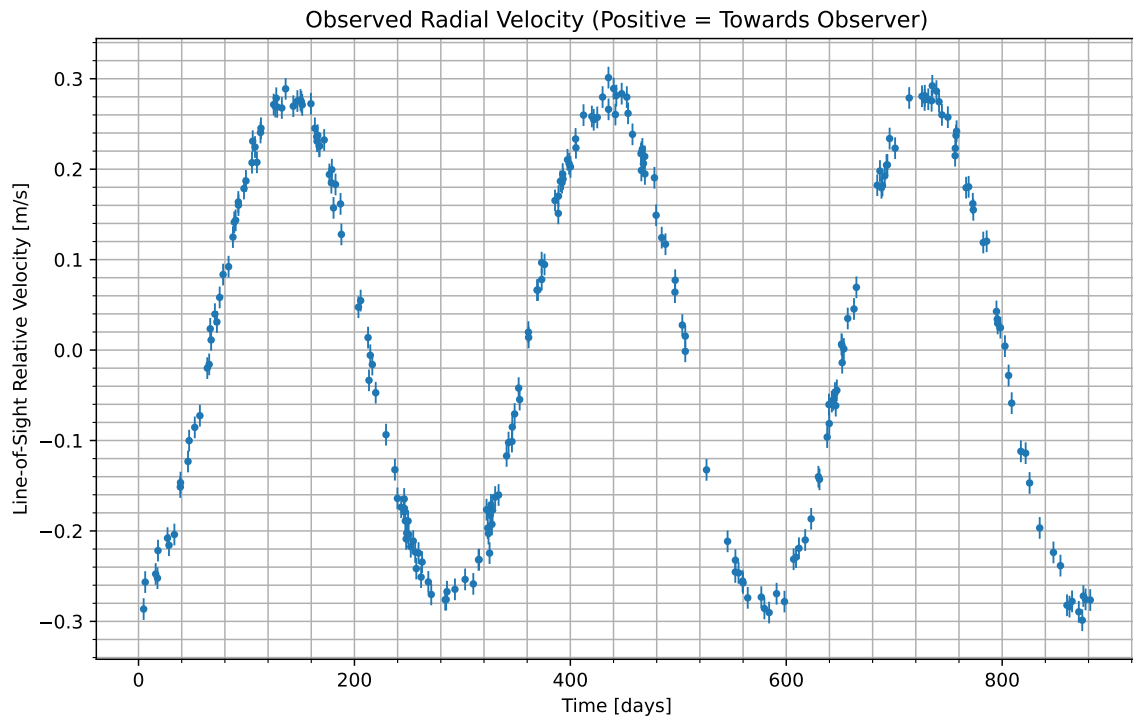
Figure 1: We have isolated the radial velocity of the host star due to the candidate planet. Data begins at UTC 2074-07-03/18:47. Positive values indicate the velocity at which the star is moving towards us; negative indicate the velocity at which it is moving away.
