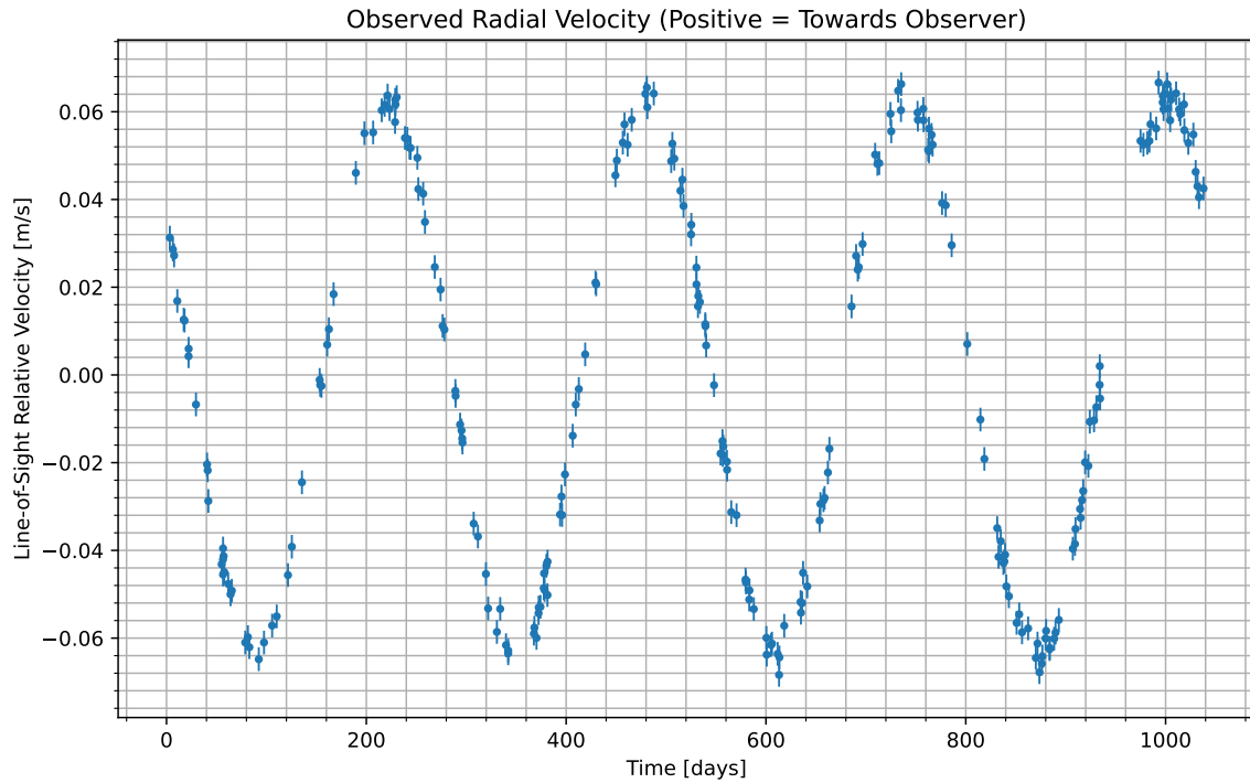
Figure 1: We have isolated the radial velocity of the host star due to the candidate planet. Data begins at UTC 2076-01-08/02:31. Positive values indicate the velocity at which the star is moving towards us; negative indicate the velocity at which it is moving away.
