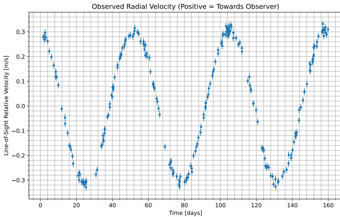
Figure 1: We have isolated the radial velocity of the host star due to the candidate planet. Data begins at UTC 2078-12-01/23:53. Positive values indicate the velocity at which the star is moving towards us; negative indicate the velocity at which it is moving away.
