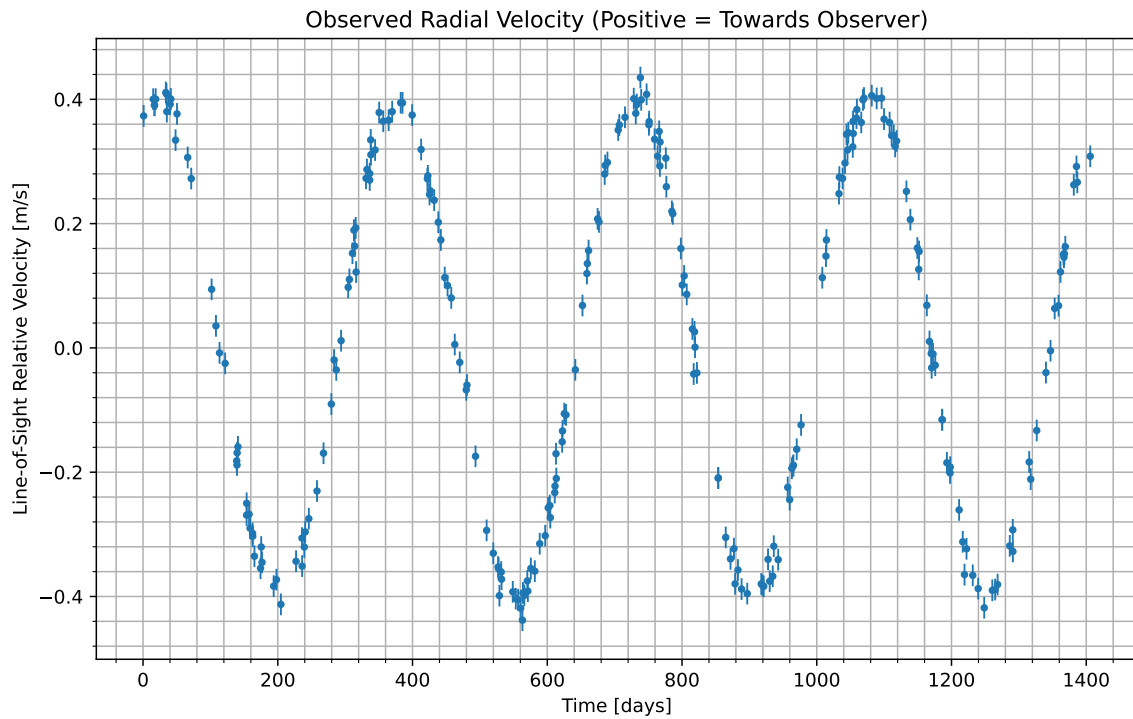
Figure 1: We have isolated the radial velocity of the host star due to the candidate planet. Data begins at UTC 2090-08-05/09:13. Positive values indicate the velocity at which the star is moving towards us; negative indicate the velocity at which it is moving away.
