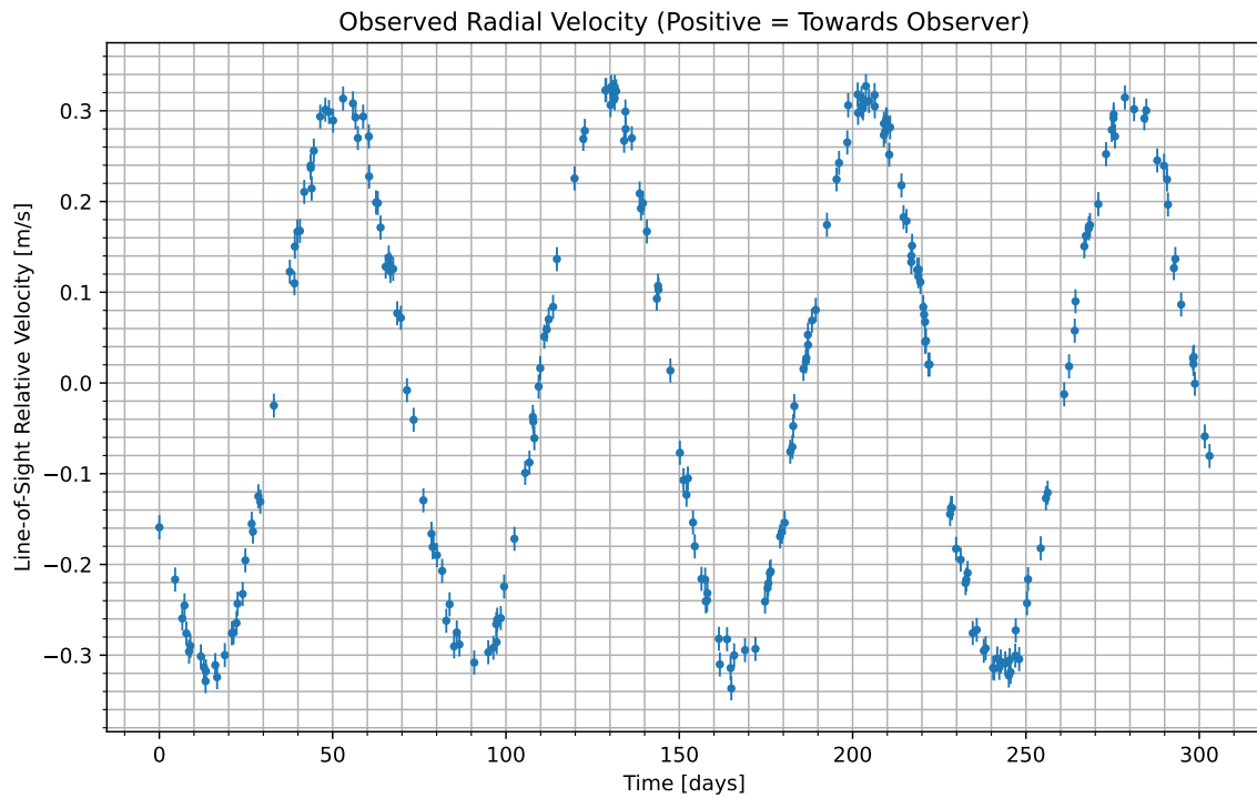
Figure 1: We have isolated the radial velocity of the host star due to the candidate planet. Data begins at UTC 2084-07-02/18:33. Positive values indicate the velocity at which the star is moving towards us; negative indicate the velocity at which it is moving away.
