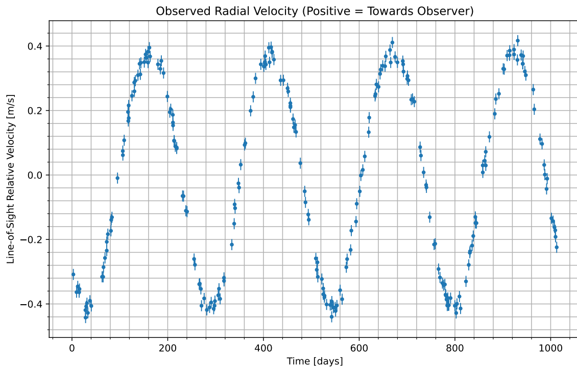
Figure 1: We have isolated the radial velocity of the host star due to the candidate planet. Data begins at UTC 2089-01-19/20:14. Positive values indicate the velocity at which the star is moving towards us; negative indicate the velocity at which it is moving away.
