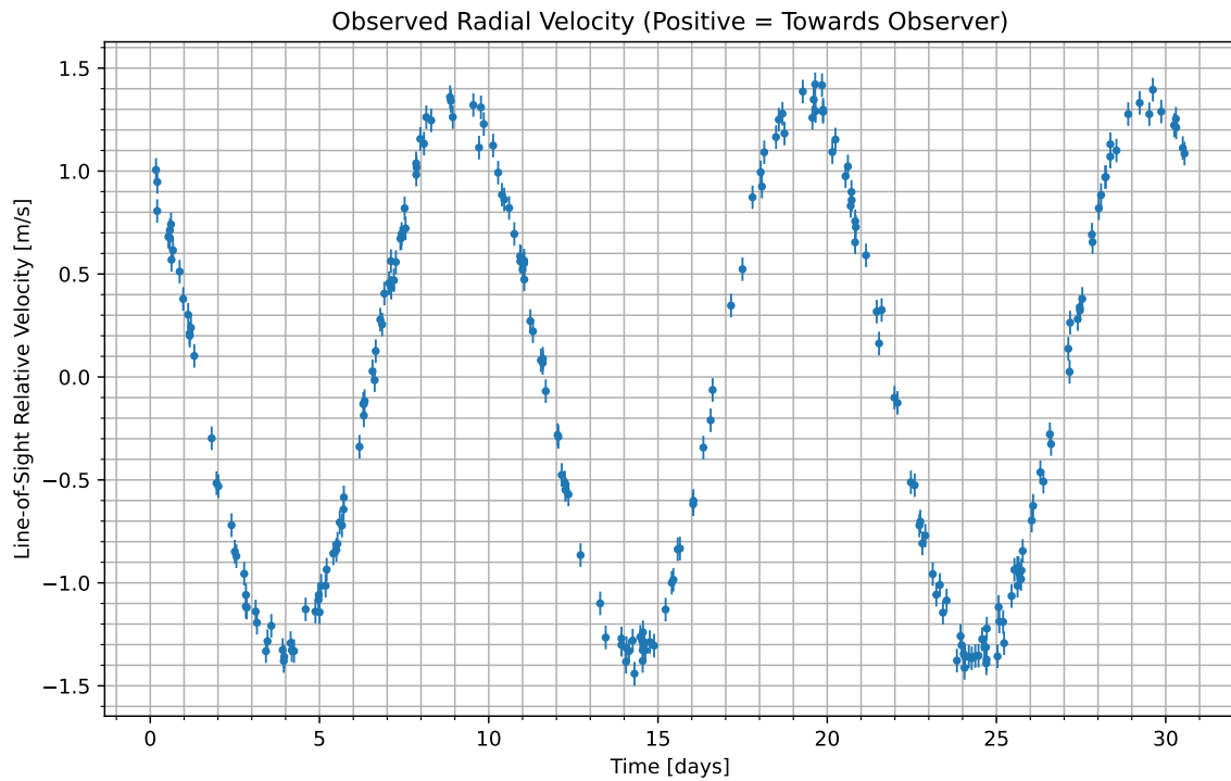
Figure 1: We have isolated the radial velocity of the host star due to the candidate planet. Data begins at UTC 2073-03-17/13:00. Positive values indicate the velocity at which the star is moving towards us; negative indicate the velocity at which it is moving away.
