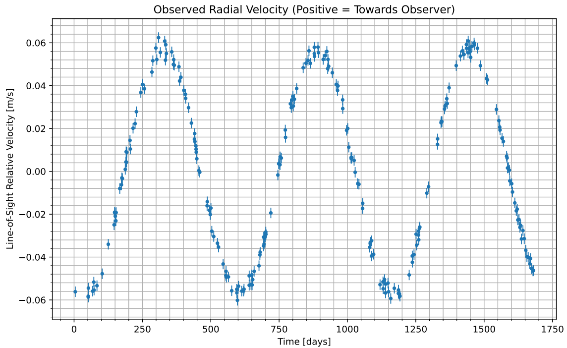
Figure 1: We have isolated the radial velocity of the host star due to the candidate planet. Data begins at UTC 2089-05-22/01:53. Positive values indicate the velocity at which the star is moving towards us; negative indicate the velocity at which it is moving away.
