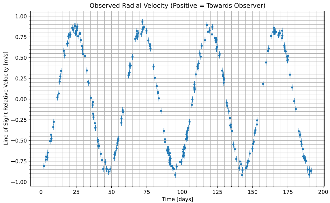
Figure 1: We have isolated the radial velocity of the host star due to the candidate planet. Data begins at UTC 2099-01-31/20:49. Positive values indicate the velocity at which the star is moving towards us; negative indicate the velocity at which it is moving away.
