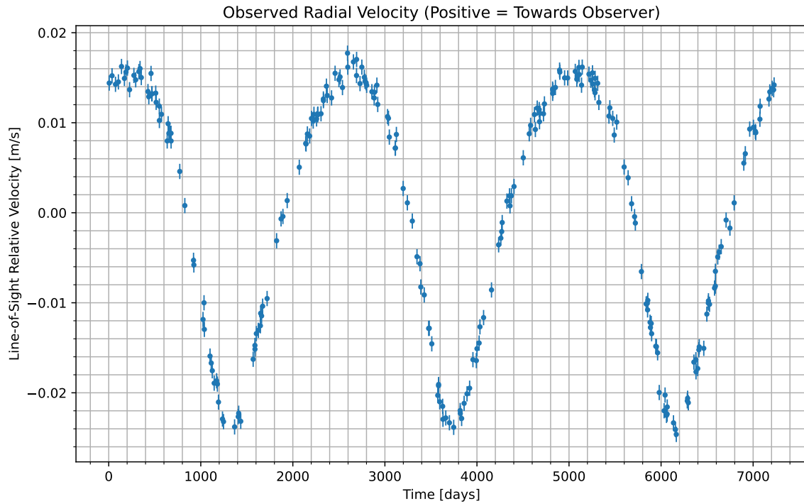
Figure 1: We have isolated the radial velocity of the host star due to the candidate planet. Data begins at UTC 2063-03-09/05:26. Positive values indicate the velocity at which the star is moving towards us; negative indicate the velocity at which it is moving away.
