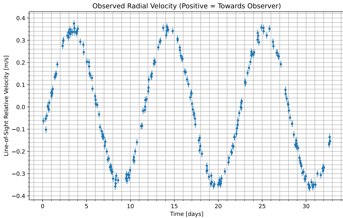
Figure 1: We have isolated the radial velocity of the host star due to the candidate planet. Data begins at UTC 2100-03-01/07:55. Positive values indicate the velocity at which the star is moving towards us; negative indicate the velocity at which it is moving away.
