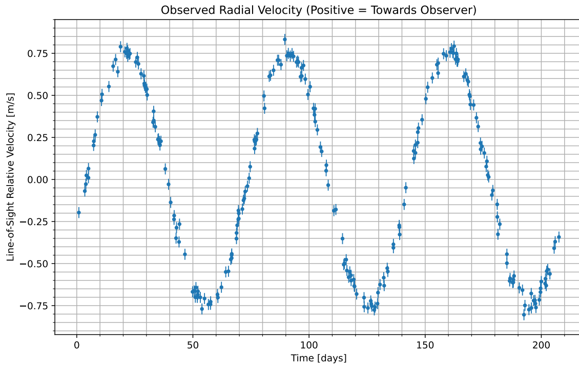
Figure 1: We have isolated the radial velocity of the host star due to the candidate planet. Data begins at UTC 2095-04-26/09:09. Positive values indicate the velocity at which the star is moving towards us; negative indicate the velocity at which it is moving away.
