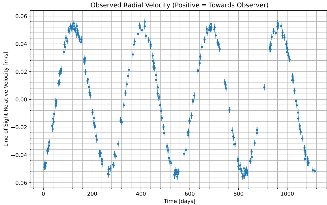
Figure 1: We have isolated the radial velocity of the host star due to the candidate planet. Data begins at UTC 2070-09-28/18:01. Positive values indicate the velocity at which the star is moving towards us; negative indicate the velocity at which it is moving away.
