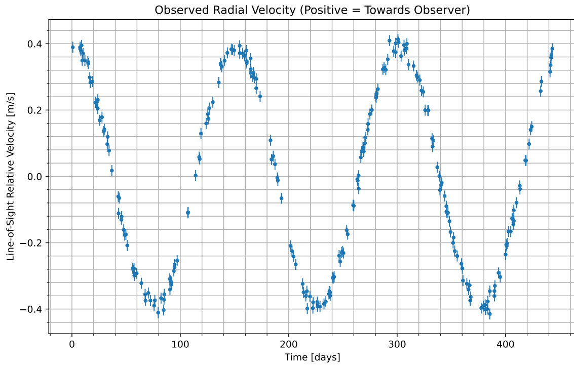
Figure 1: We have isolated the radial velocity of the host star due to the candidate planet. Data begins at UTC 2090-07-02/20:00. Positive values indicate the velocity at which the star is moving towards us; negative indicate the velocity at which it is moving away.
