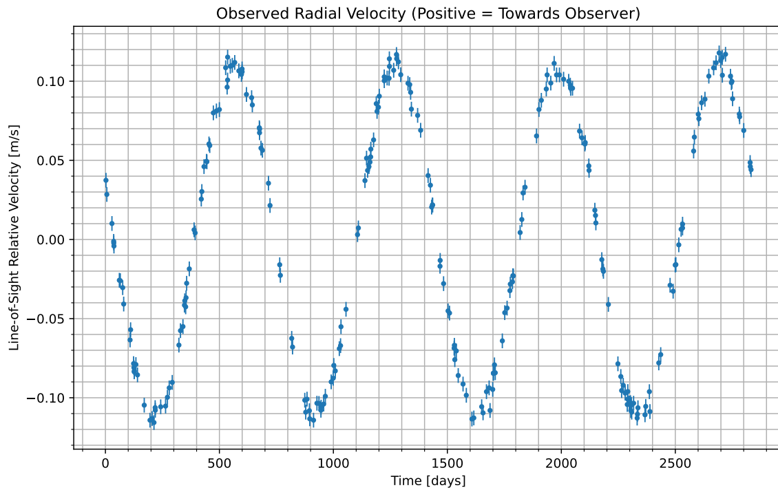
Figure 1: We have isolated the radial velocity of the host star due to the candidate planet. Data begins at UTC 2089-11-22/02:07. Positive values indicate the velocity at which the star is moving towards us; negative indicate the velocity at which it is moving away.
