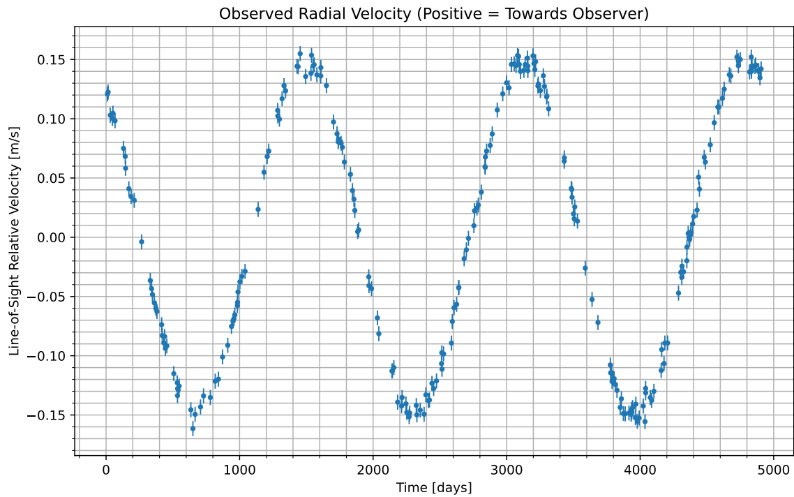
Figure 1: We have isolated the radial velocity of the host star due to the candidate planet. Data begins at UTC 2057-07-19/19:04. Positive values indicate the velocity at which the star is moving towards us; negative indicate the velocity at which it is moving away.
