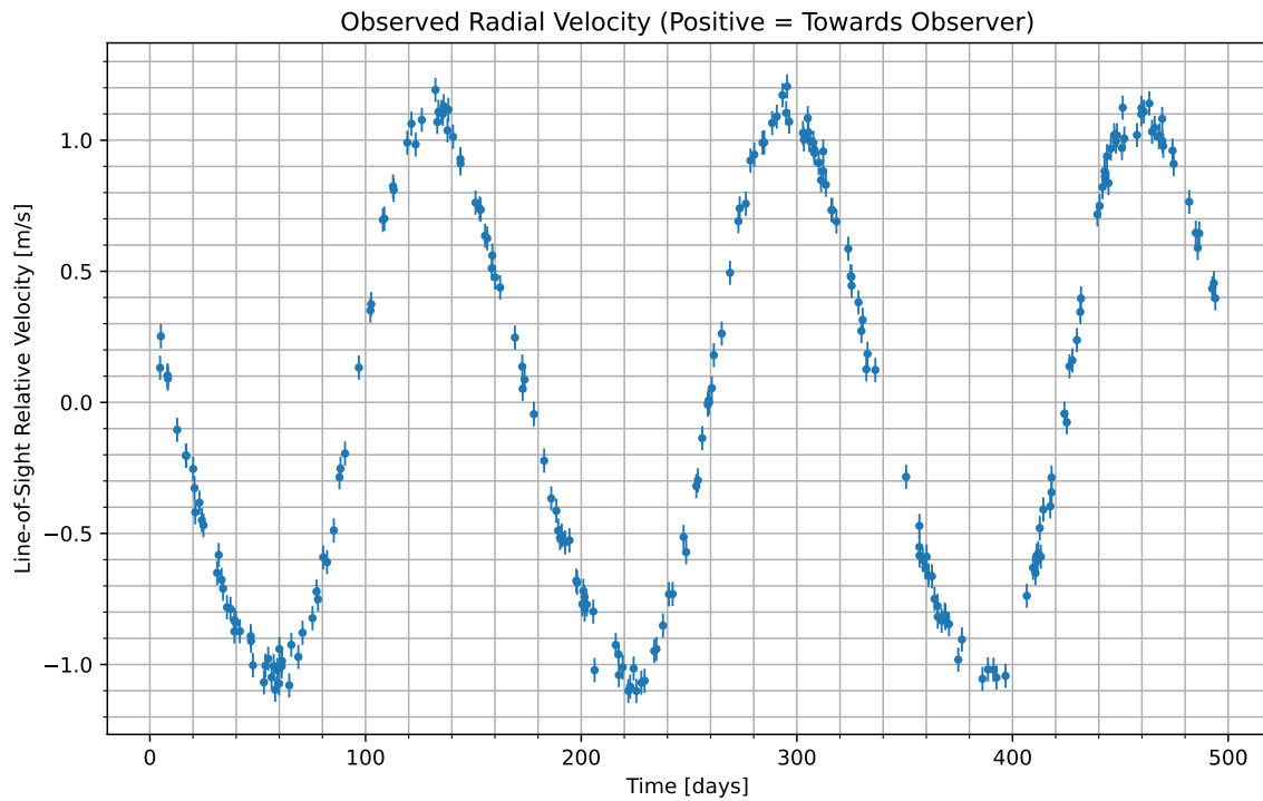
Figure 1: We have isolated the radial velocity of the host star due to the candidate planet. Data begins at UTC 2080-09-09/04:51. Positive values indicate the velocity at which the star is moving towards us; negative indicate the velocity at which it is moving away.
