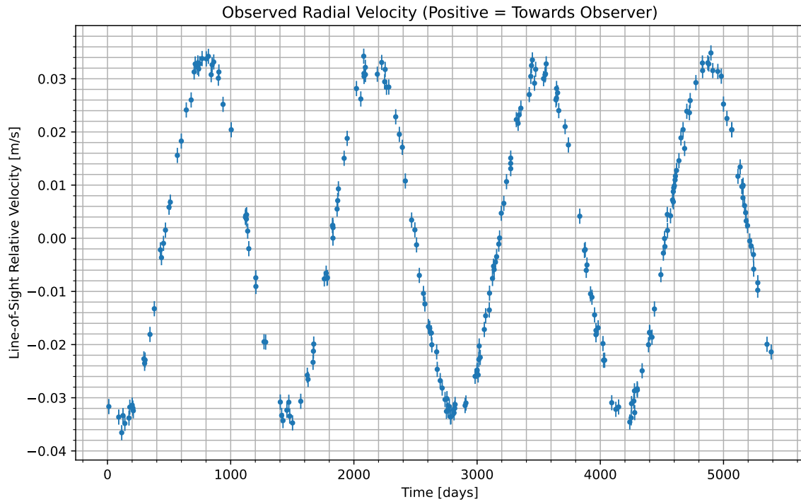
Figure 1: We have isolated the radial velocity of the host star due to the candidate planet. Data begins at UTC 2069-06-12/06:53. Positive values indicate the velocity at which the star is moving towards us; negative indicate the velocity at which it is moving away.
