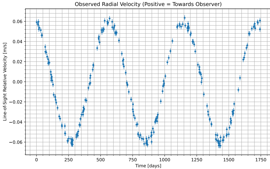
Figure 1: We have isolated the radial velocity of the host star due to the candidate planet. Data begins at UTC 2069-03-20/20:16. Positive values indicate the velocity at which the star is moving towards us; negative indicate the velocity at which it is moving away.
